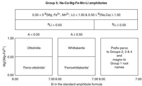
FIGURE 3. Classification of the Group 5 amphiboles; Na-Ca-Mg-Fe-Mn-Li amphiboles.
