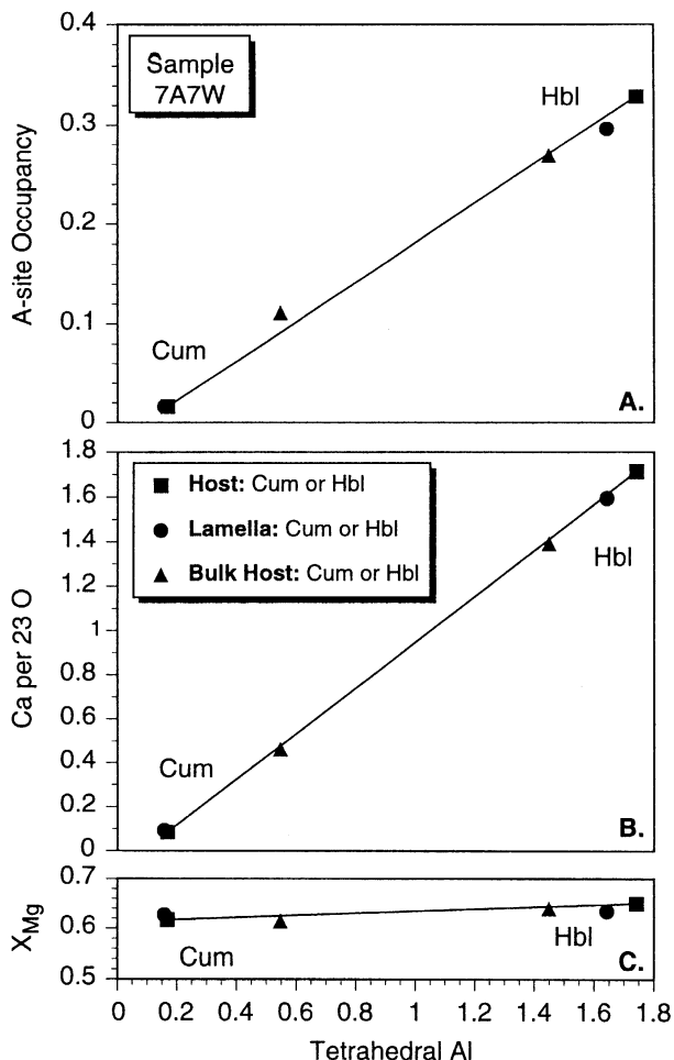
FIGURE 2. Three chemical plots of coexisting clin amphiboles (sample 7A7W). (A) ^{14}\text{Al} vs. A-site occupancy, (B) ^{14}\text{Al} vs. Ca per 23 O atoms, and (C) ^{14}\text{Al} vs. X_{\text{Mg}} . The bulk compositions of the host phases are averages of 60–70 electron microprobe point analyses across a single grain. Host and lamellar compositions were averages of 10–15 point analyses.
