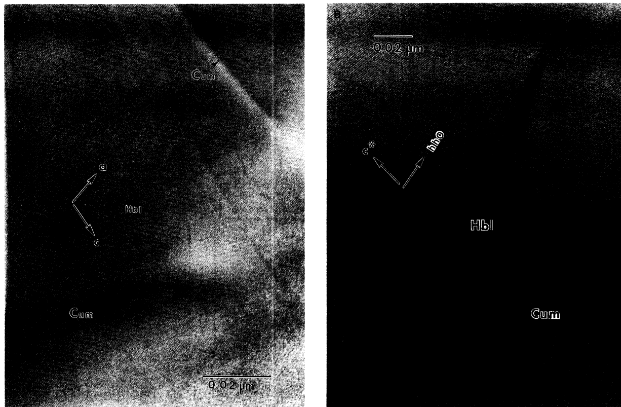
FIGURE 5. (A) HRTEM image of sample WD-H26C showing the coherent intergrowth between hornblende (Hbl) host and cummingtonite (Cum) exsolution lamellae. (B) HRTEM image of sample Q-603C showing the coherent intergrowth between cummingtonite host and “10 \bar{1} ” hornblende disc-shaped exsolution lamella viewed along [1 \bar{1} 0].
