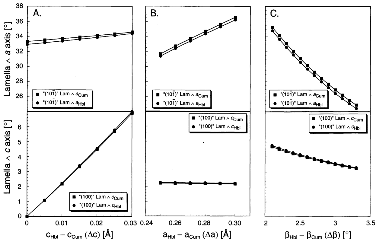
FIGURE 6. OPB calculations with constant a and \beta (A), constant c and \beta (B), and constant a and c (C). Lattice parameters used are a_{\text{Cum}} = 9.54 \text{ \AA} , c_{\text{Cum}} = 5.35 \text{ \AA} , \beta_{\text{Cum}} = 102.22^\circ , a_{\text{Hbl}} = 9.81 \text{ \AA} , c_{\text{Hbl}} = 5.35 \text{ \AA} , and \beta_{\text{Hbl}} = 104.67^\circ .
