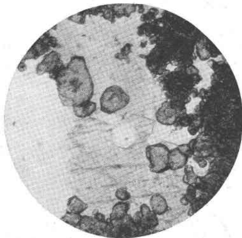
FIG. 4. Another portion of the garnet phase showing a basal section of quartz surrounded by calcite. Snoqualmie Pass, Washington. 35X.
