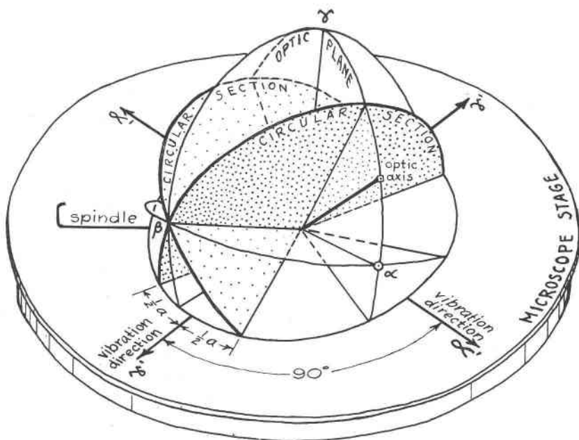
FIG. 3. Vibration directions in a biaxial crystal with the symmetry axes of the indicatrix inclined to the microscope stage and spindle axis.
