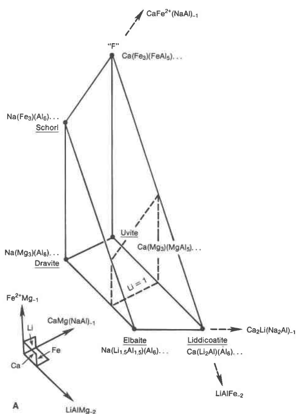
Fig. 3. Vector representation of tourmaline compositions derived from dravite by operation of the vectors \text{CaMg(NaAl)}_{-1} (horizontal) and \text{LiAlMg}_{-2} (vertical).
