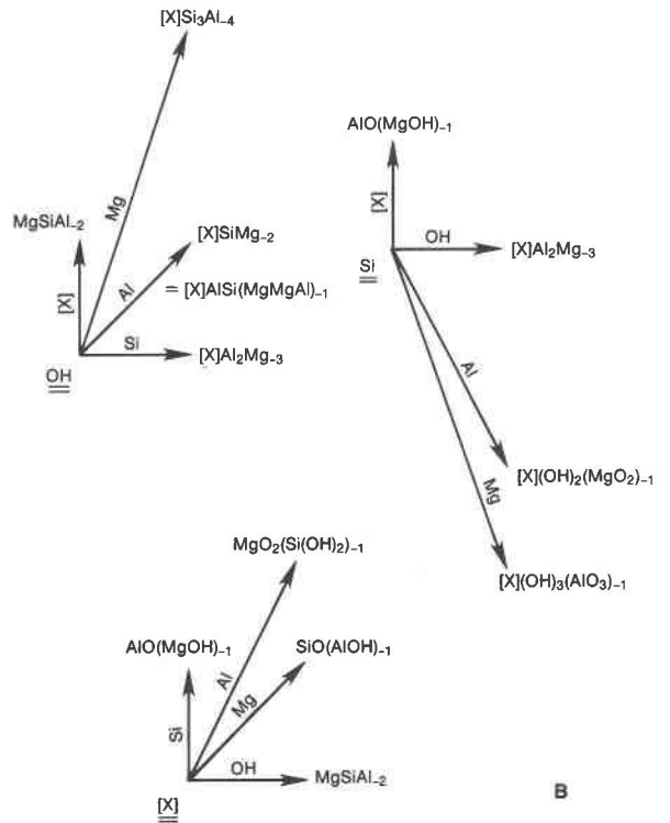
Fig. 20. Composition volume for alkali-free tourmalines. (A) Tourmaline compositions derived from "M" (magnesian analogue of uvite) by operation of the vectors [X]Al_2Mg_{-3} (lower right), MgSiAl_{-2} (lower left), and AIO(MgOH)_{-1} (vertical), where [X] refers to an X-site vacancy. "S" is as in Fig. 12. Plane sloping toward the right front has Mg = 0 . (B) Basis and derived vectors for planes of constant OH, Si, and [X] in Fig. 20A.
