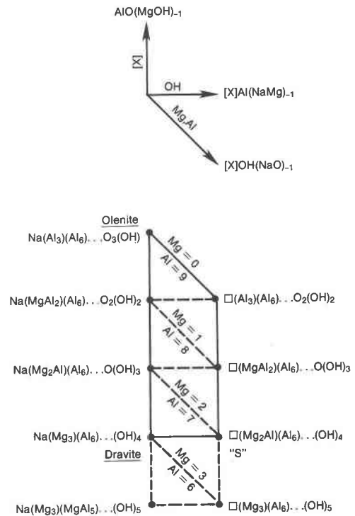
Fig. 12. Tourmaline compositions derived from dravite by operation of the vectors [X]Al(NaMg)_{-1} (horizontal) and AIO(MgOH)_{-1} (vertical), where [X] is an X-site vacancy. "S" is the approximate composition of a synthetic alkali-free tourmaline prepared by Rosenberg and Foit (1975) and Werding and Schreyer (1984).
