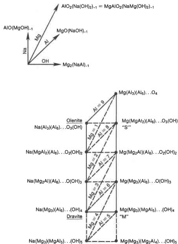
Fig. 13. Tourmaline compositions derived from dravite by operation of the vectors Mg_2(NaAl)_{-1} (horizontal) and AlO(MgOH)_{-1} (vertical). "M" corresponds to a magnesian analogue of uvite; "S" is a magnesian tourmaline synthesized by Rosenberg and Foit (1975).
