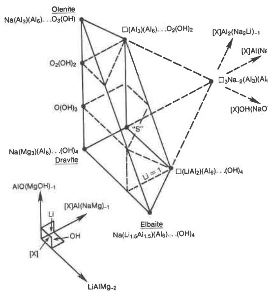
Fig. 15. Tourmaline compositions derived from dravite by operation of the three vectors [X]Al(NaMg)_{-1} (upper right), LiAlMg_{-2} (lower right), and AlO(MgOH)_{-1} (vertical). "S" is as in Fig. 12.
