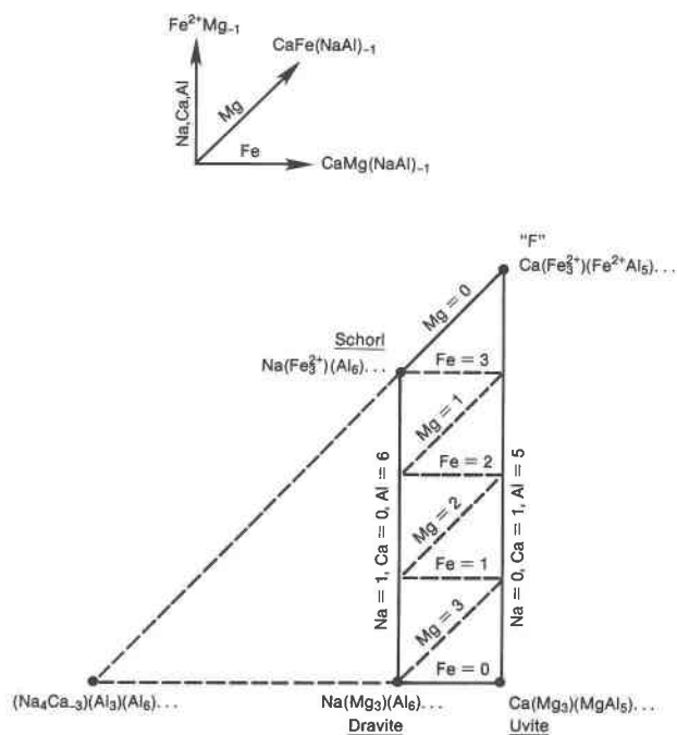
Fig. 2. Vector representation of tourmaline compositions derived from dravite by operation of the vectors \text{CaMg}(\text{NaAl})_{-1} (horizontal) and \text{FeMg}_{-1} (vertical). "F" = hypothetical ferrous end-member.
