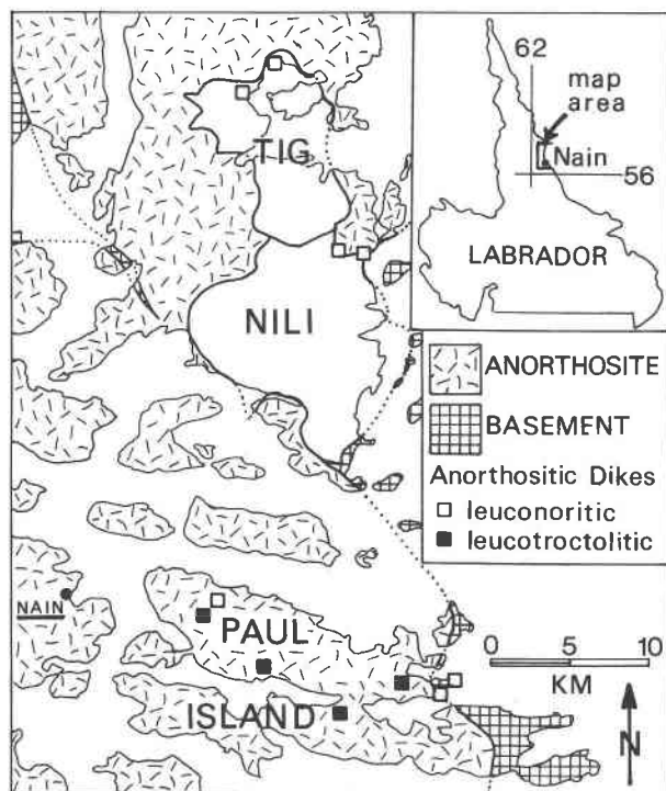
Fig. 1. Index map and simplified geologic map of a portion of the Nain complex. TIG = Tigalak layered intrusion (Wiebe and Wild, 1983). NILI = Newark Island layered intrusion (Wiebe, 1988b).
