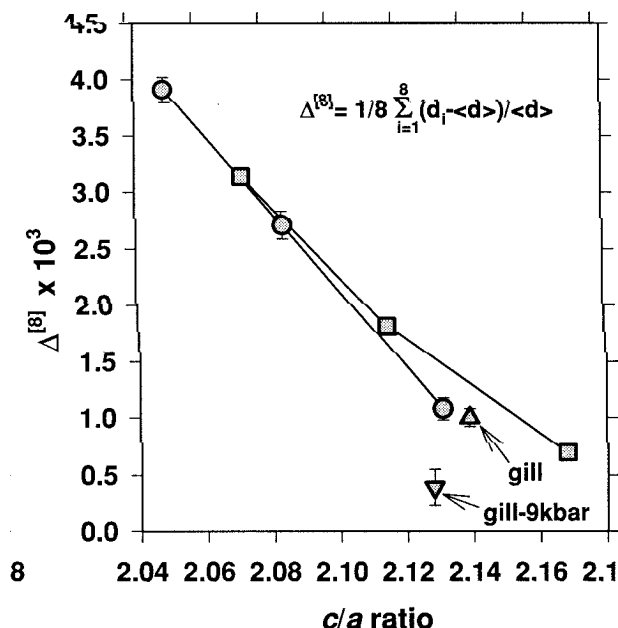
FIGURE 7. Variation of the \text{AO}_8 bond-length distortion parameter \Delta^{[8]} (Brown and Shannon 1973). \langle d \rangle = mean A-O bond distance; symbol notation: see Figure 2.
