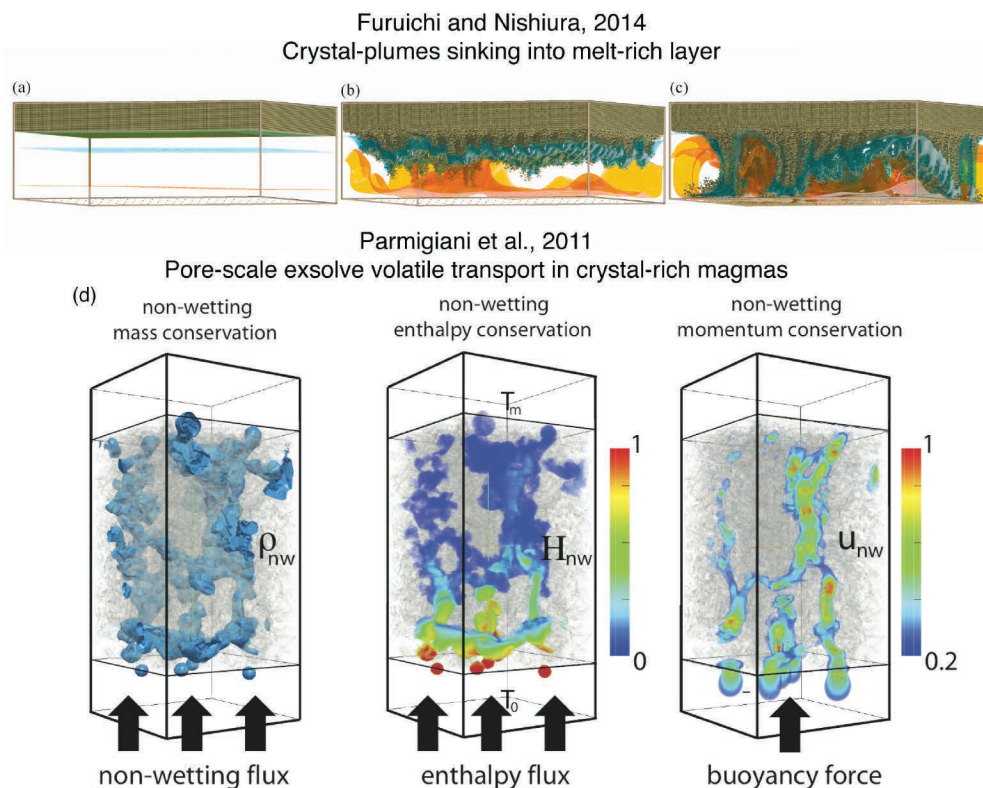
FIGURE 4. Example of granular scale calculation for multiphase magma chamber dynamics. (a–c) modified from from Furuichi and Nishiura (2014) for crystal settling from a stratified chamber with a crystal-free region at the bottom and a denser, crystal-rich horizon, at the top, and (d) Parmigiani et al. 2011 for the migration of a buoyant volatile phase in a crystal-rich rigid magma.
